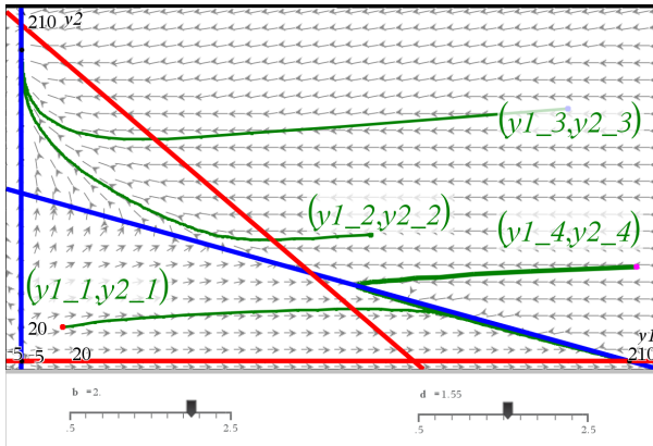
Figure 15: case 1
