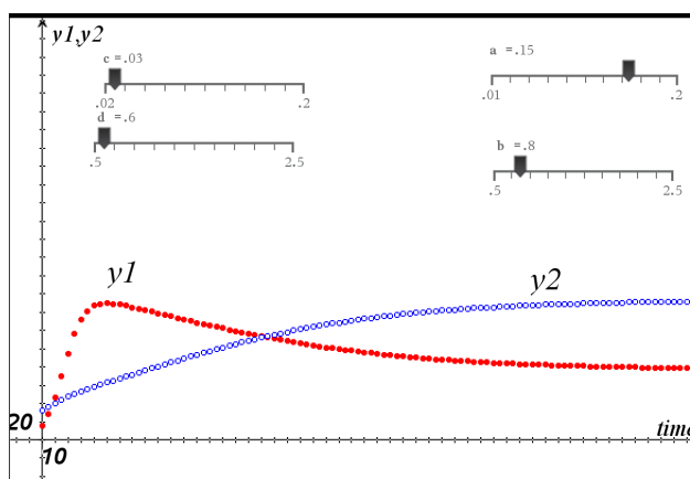
Figure 11: time-graph of y1 and y2
