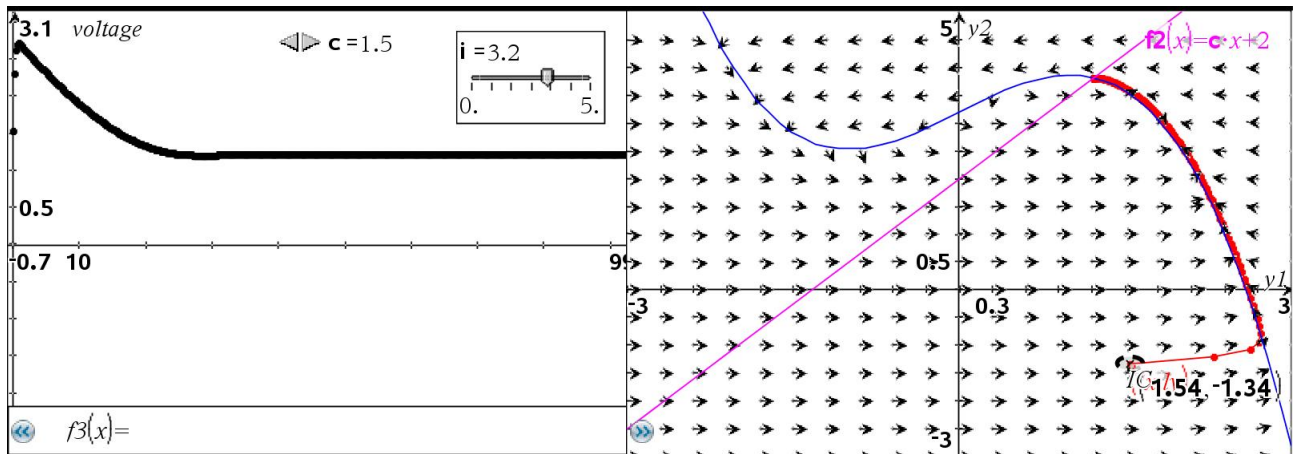
Figure 23: Stimulus I = 3.2
