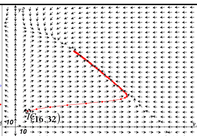
Figure 12: trajectory
