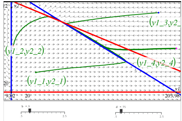
Figure 16: case 2
