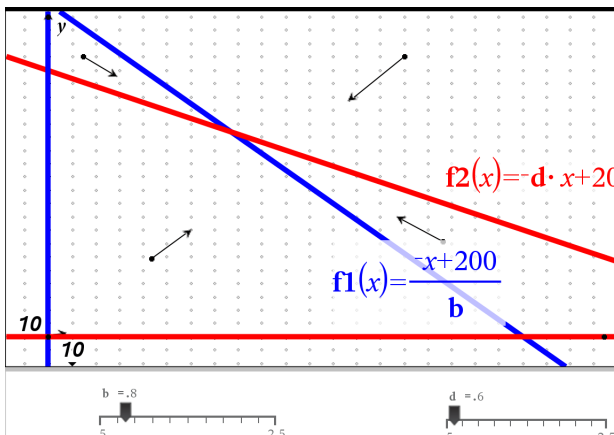
Figure 13: nullclines and isosectors
