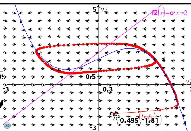
Figure 22: limit cycle
