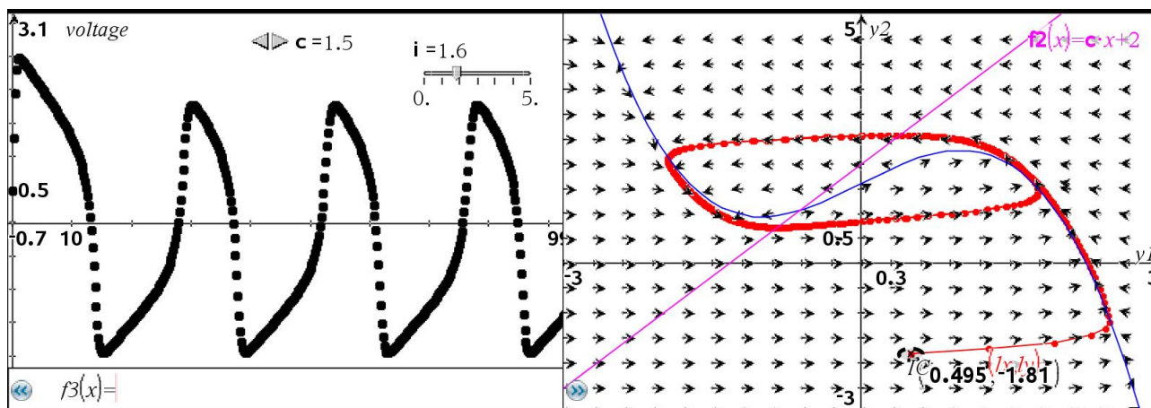
Figure 21: Stimulus I = 1.6
