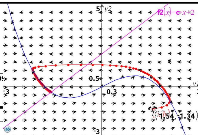
Figure 20: stable equilibrium
