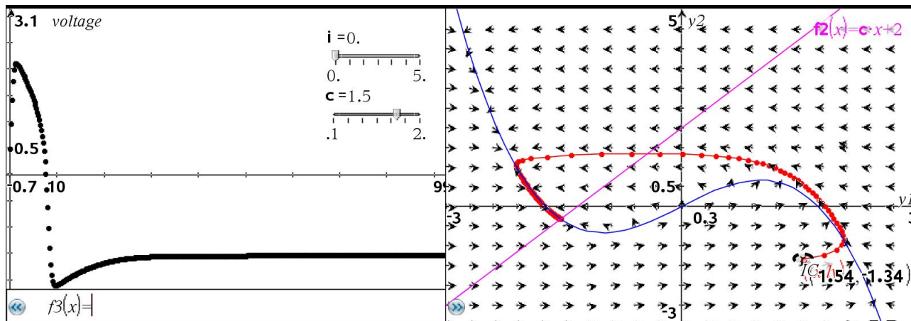
Figure 19: Stimulus I = 0
