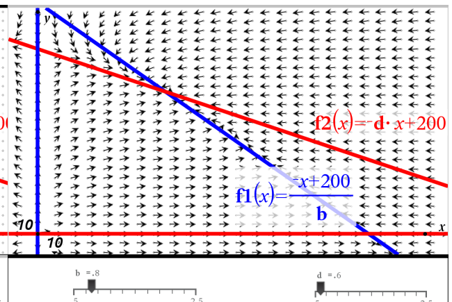
Figure 14: direction field
